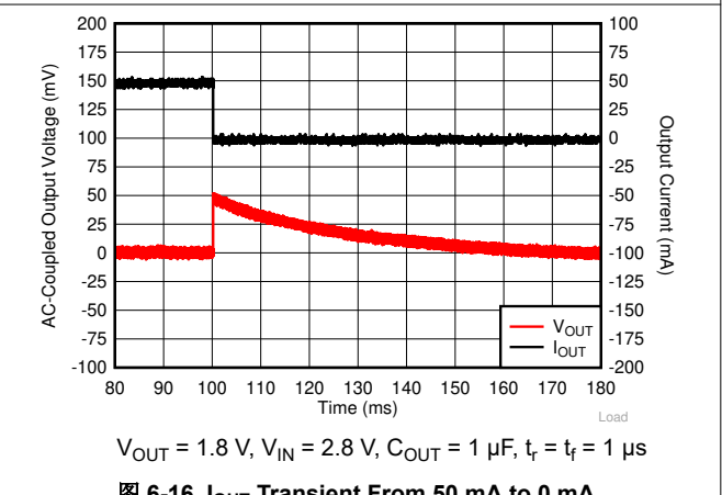
图 6-16. I_{OUT} Transient From 50 mA to 0 mA
