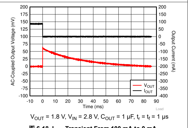
图 6-18. I_{OUT} Transient From 100 mA to 0 mA
