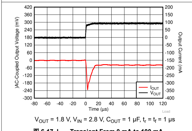
图 6-17. I_{OUT} Transient From 0 mA to 100 mA
