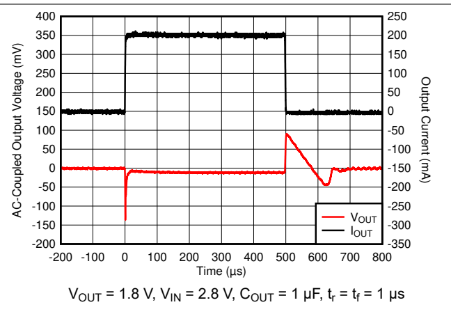
图 6-14. I_{OUT} Transient From 1 mA to 200 mA
