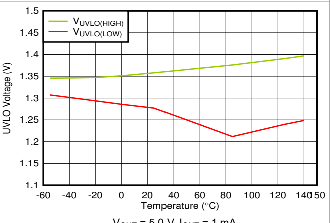
图 6-40. UVLO Rising and Falling Threshold vs Temperature
