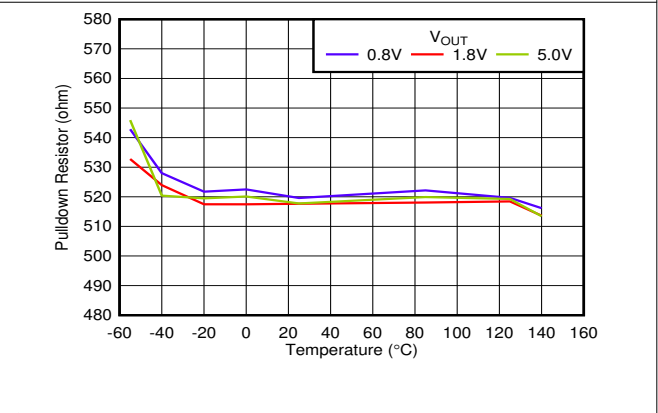
图 6-42. Smart Enable Pulldown Resistor vs Temperature and V_{OUT}
