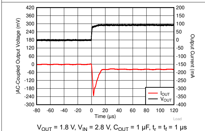
图 6-17. I_{OUT} Transient From 0 mA to 100 mA
