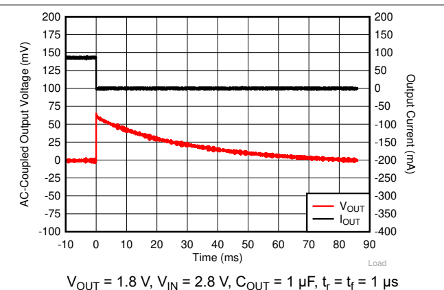
图 6-18. I_{OUT} Transient From 100 mA to 0 mA
