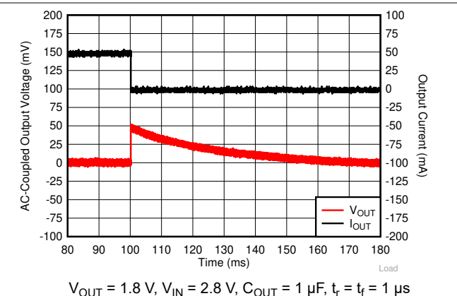
图 6-16. I_{OUT} Transient From 50 mA to 0 mA
