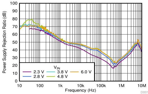
图 6-45. PSRR vs Frequency and V_{IN} V_{OUT} = 1.8\text{ V} , I_{OUT} = 100\text{ mA} , C_{OUT} = 1\text{ }\mu\text{F}
