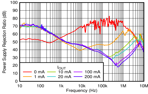
图 6-43. PSRR vs Frequency and I_{OUT} V_{IN} = 2.8\text{ V} , V_{OUT} = 1.8\text{ V} , C_{OUT} = 1\text{ }\mu\text{F}
