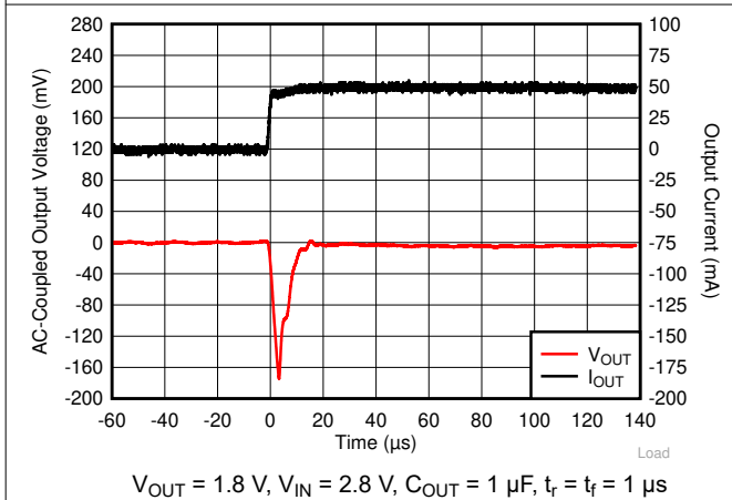
图 6-15. I_{OUT} Transient From 0 mA to 50 mA
