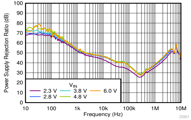
图 6-44. PSRR vs Frequency and V_{IN} V_{OUT} = 1.8\text{ V} , I_{OUT} = 20\text{ mA} , C_{OUT} = 1\text{ }\mu\text{F}
