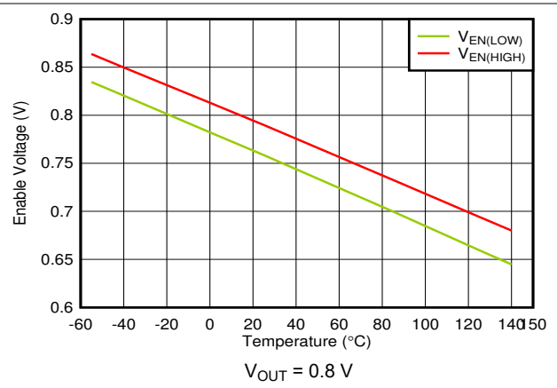
图 6-38. EN High and Low Threshold vs Temperature
