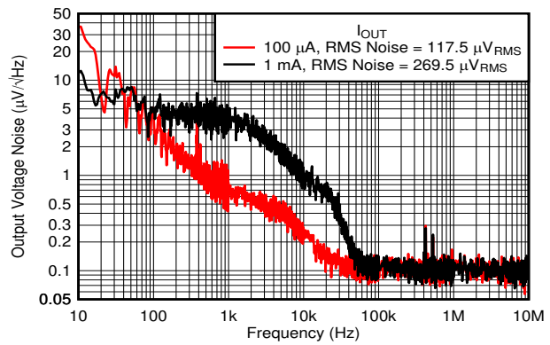
图 6-48. Output Noise vs Frequency and I_{OUT} V_{OUT} = 1.8\text{ V} , V_{IN} = 2.8\text{ V} , C_{OUT} = 1\text{ }\mu\text{F}
