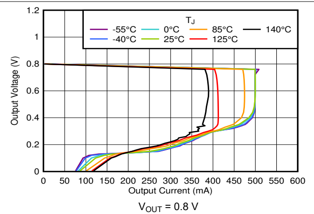
图 6-36. Foldback Current Limit vs I_{OUT} and Temperature
