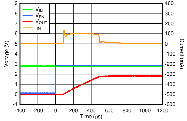
图 6-56. Startup Inrush Current With C_{OUT} = 22\text{ }\mu\text{F}
