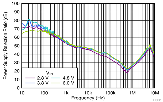
图 6-46. PSRR vs Frequency and V_{IN} V_{OUT} = 1.8\text{ V} , I_{OUT} = 200\text{ mA} , C_{OUT} = 1\text{ }\mu\text{F}
