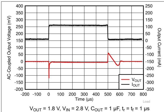
图 6-13. I_{OUT} Transient From 1 mA to 100 mA
