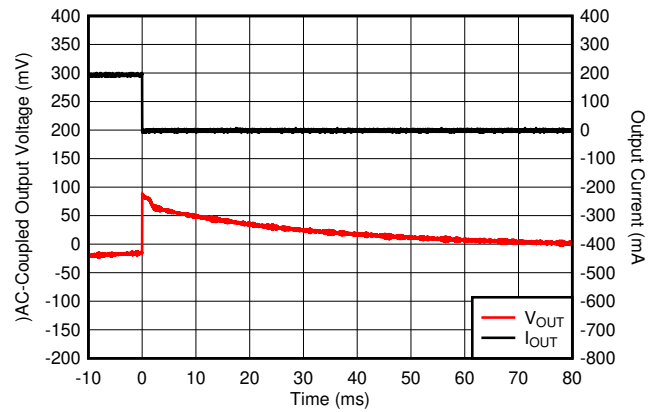
图 6-20. I_{OUT} Transient From 200 mA to 0 mA
