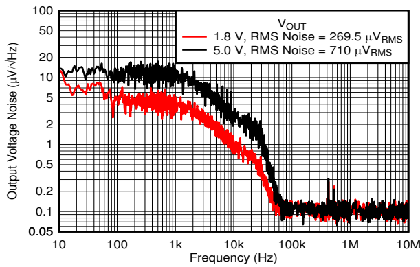
图 6-47. Output Noise vs Frequency and V_{OUT}
