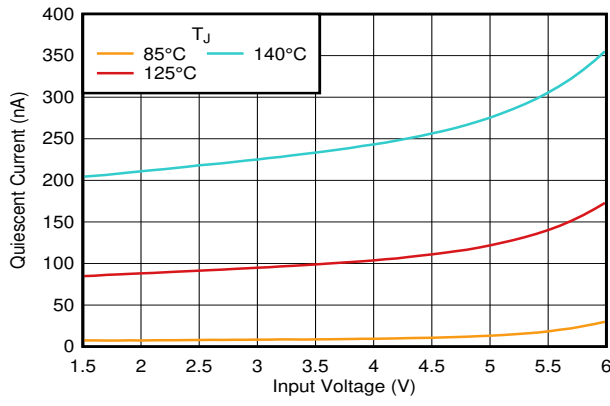
图 6-11. I_{SHDN} vs V_{IN} and Temperature
