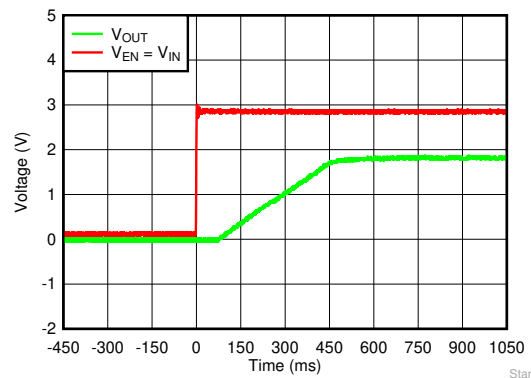
图 6-50. Startup With V_{EN} = V_{IN}
