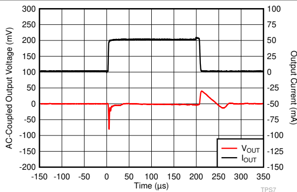
V_{OUT} = 1.8\text{ V} , V_{IN} = 2.8\text{ V} , C_{OUT} = 1\text{ }\mu\text{F} , t_r = t_f = 1\text{ }\mu\text{s} 图 6-13. I_{OUT} Transient From 1 mA to 50 mA
