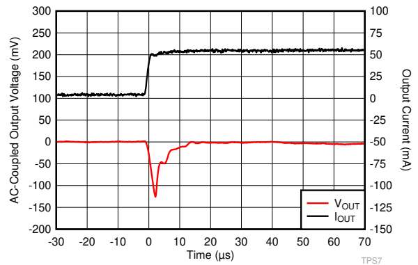
V_{OUT} = 1.8\text{ V} , V_{IN} = 2.8\text{ V} , C_{OUT} = 1\text{ }\mu\text{F} , t_r = t_f = 1\text{ }\mu\text{s} 图 6-16. I_{OUT} Transient From 0 mA to 50 mA
