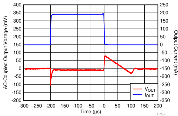
V_{OUT} = 1.8\text{ V} , V_{IN} = 2.8\text{ V} , C_{OUT} = 1\text{ }\mu\text{F} , t_r = t_f = 1\text{ }\mu\text{s} 图 6-15. I_{OUT} Transient From 1 mA to 200 mA
