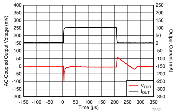
V_{OUT} = 1.8\text{ V} , V_{IN} = 2.8\text{ V} , C_{OUT} = 1\text{ }\mu\text{F} , t_r = t_f = 1\text{ }\mu\text{s} 图 6-14. I_{OUT} Transient From 1 mA to 100 mA
