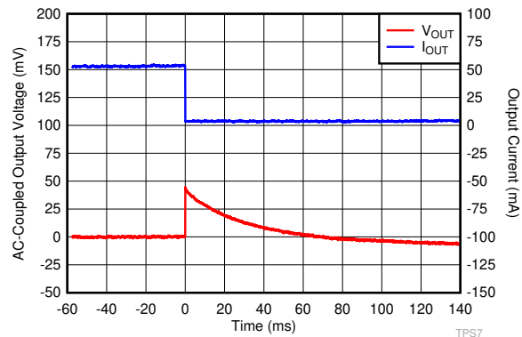
V_{OUT} = 1.8\text{ V} , V_{IN} = 2.8\text{ V} , C_{OUT} = 1\text{ }\mu\text{F} , t_r = t_f = 1\text{ }\mu\text{s} 图 6-17. I_{OUT} Transient From 50 mA to 0 mA
