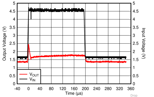
图 6-25. V_{IN} Transient From 1.5 V to 4.5 V
