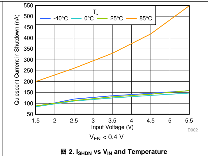
图 2. I_{SHDN} vs V_{IN} and Temperature
