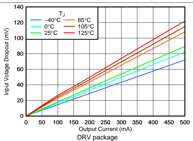
图 4. V_{IN} Dropout vs I_{OUT} and Temperature
