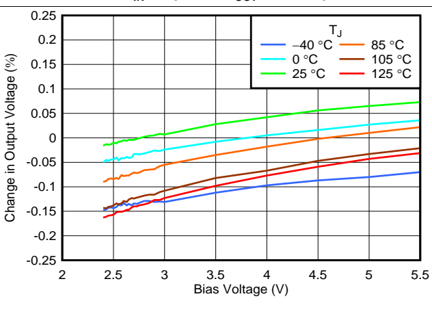
图 6. Output Accuracy vs V_{BIAS} and Temperature
