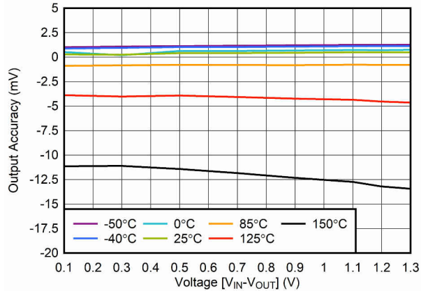
图 6-1. Output Voltage Accuracy vs V_{IN}
