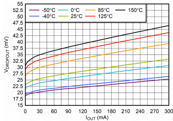
图 8-5. V IN Dropout Voltage vs I OUT
