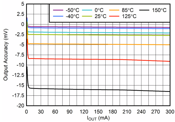
图 6-3. Output Voltage Accuracy vs I_{OUT}
