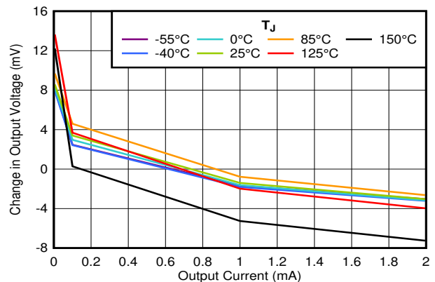
V_{IN} = 3.1\text{ V} , V_{EN} = 1\text{ V} , DQN, YCJ, and YCK packages
