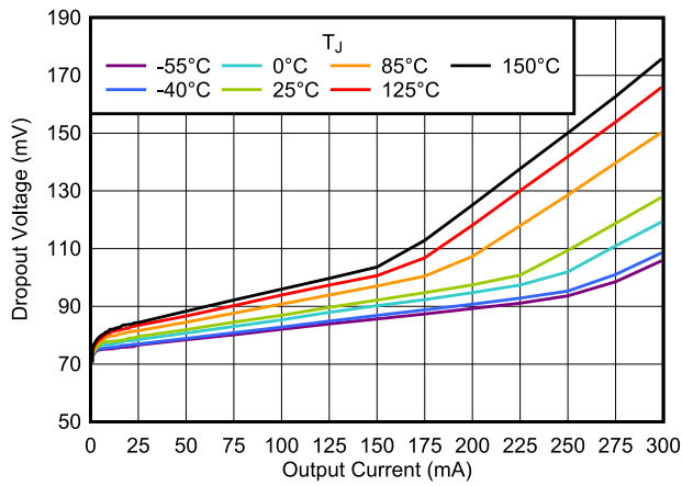
图 6-31. Dropout Voltage vs I_{OUT}
