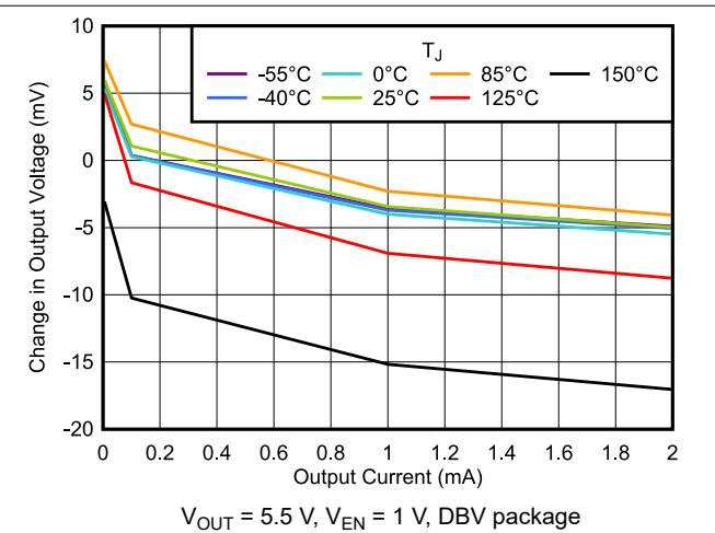
图 6-12. Load Regulation vs I_{OUT}
