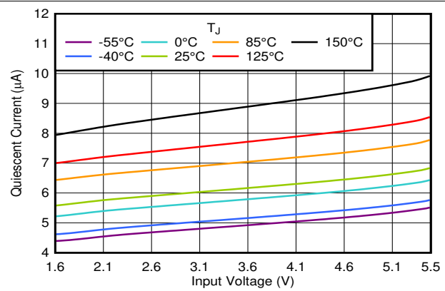
图 6-36. I_{GND} vs V_{IN} in the Dropout Region
