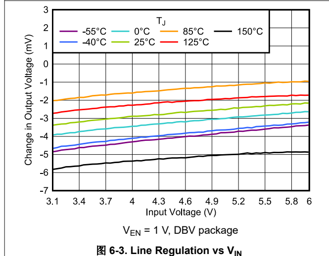
图 6-3. Line Regulation vs V_{IN}
