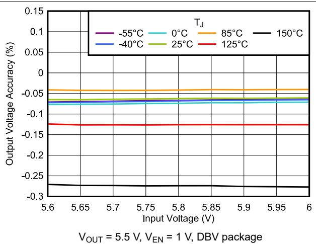
图 6-24. Output Voltage Accuracy vs V_{IN}
