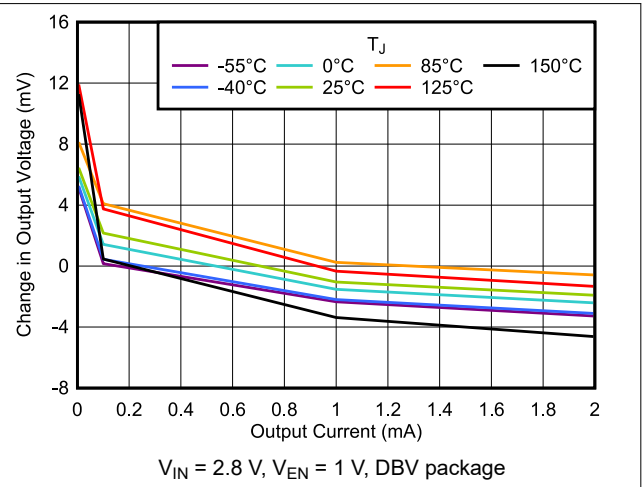
图 6-8. Load Regulation vs I_{OUT}
