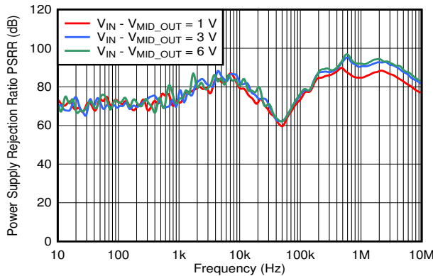
C_{IN} = 0\text{ }\mu\text{F} , V_{OUT} = 3.3\text{ V} , I_{OUT} = 20\text{ mA}
