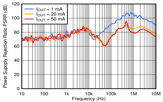
V_{IN} = 13\text{ V} , C_{IN} = 0\text{ }\mu\text{F} , V_{OUT} = 3.3\text{ V}
