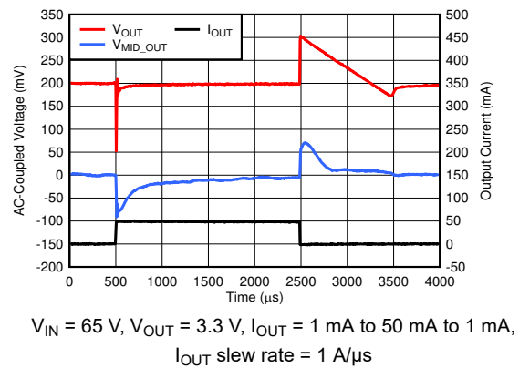
Figure 6-24. Load Transient
