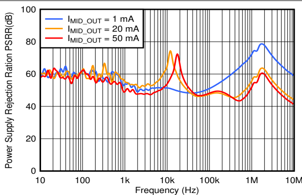
V_{IN} = 13\text{ V} , C_{IN} = 0\text{ }\mu\text{F} , V_{OUT} = 3.3\text{ V} , I_{OUT} = 0\text{ mA}
