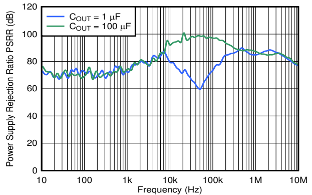
V_{IN} = 13\text{ V} , C_{IN} = 0\text{ }\mu\text{F} , V_{OUT} = 3.3\text{ V} , I_{OUT} = 20\text{ mA}
