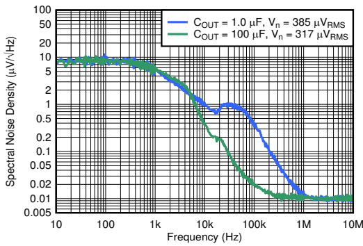
V_{IN} = 13\text{ V} , V_{OUT} = 3.3\text{ V} , I_{OUT} = 20\text{ mA} , V_{RMS} bandwidth = 10 Hz to 100 kHz
