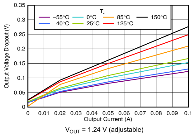
Figure 6-10. V_{\text{DO(OUT)}} vs I_{\text{OUT}}
