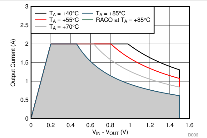
图 9-20. Recommended Area for Continuous Operation for V_{OUT} = 5\text{ V}
