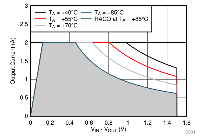
图 9-18. Recommended Area for Continuous Operation for V_{OUT} = 2.5\text{ V}
