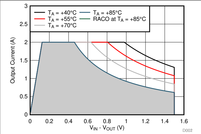
图 9-16. Recommended Area for Continuous Operation for V_{OUT} = 1.2\text{ V}
