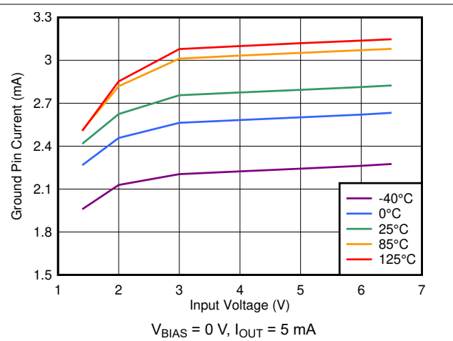
图 7-32. Ground Pin Current vs Input Voltage
