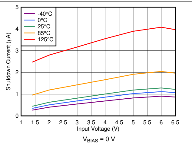
图 7-34. Shutdown Current vs Input Voltage
