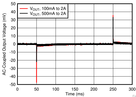
图 7-19. Load Transient vs Time and DC Load
