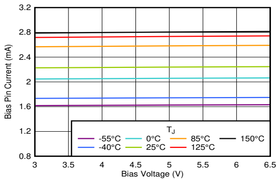
图 6-79. Bias Pin Current With Bias
