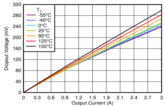
图 6-70. Dropout Voltage vs I_{OUT} (High V_{IN} ) V_{IN} = 5.6\text{ V}
