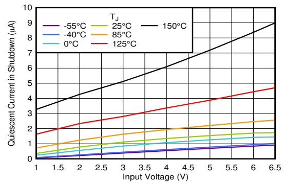
图 6-80. Shutdown Current vs V_{IN}
