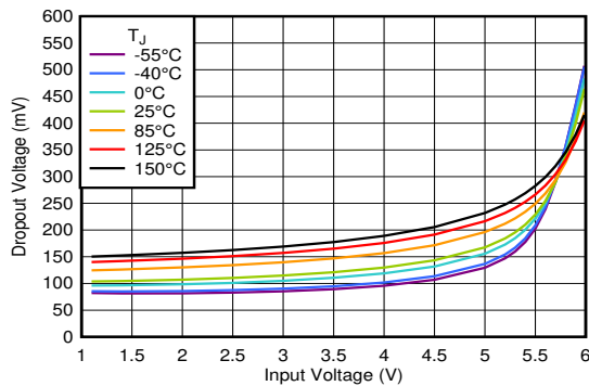
图 6-67. Dropout Voltage vs V_{IN} With Bias I_{OUT} = 3\text{ A} , V_{BIAS} = 5.0\text{ V}
