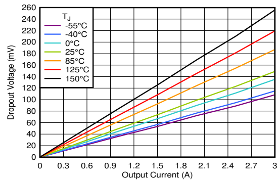
图 6-68. Dropout Voltage vs I_{OUT} Without Bias V_{IN} = 1.4\text{ V}
