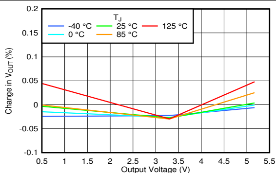
图 6-71. Load Regulation vs V_{OUT} I_{OUT} = 100\text{ mA to }3\text{ A}
