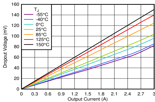
图 6-69. Dropout Voltage vs I_{OUT} With Bias V_{IN} = 1.1\text{ V} , V_{BIAS} = 5.0\text{ V}
