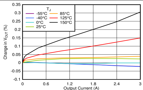
图 6-72. Load Regulation vs I_{OUT} V_{IN} = 1.4\text{ V}
