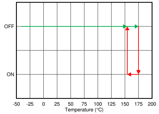
Figure 6-38. Thermal Shutdown
