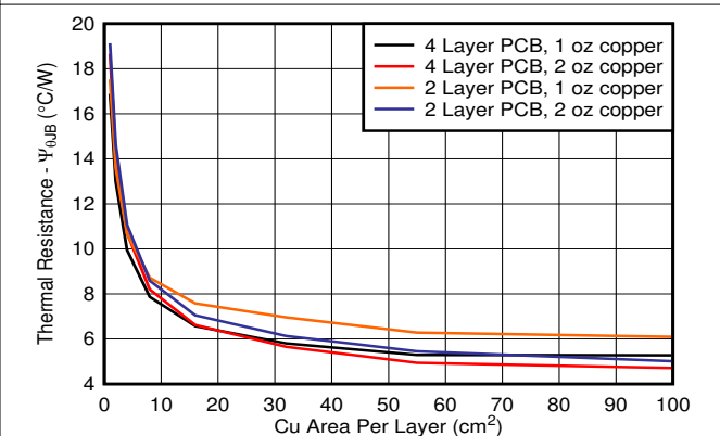
图 8-5. \psi_{JB} vs Copper Area (KVU Package)
