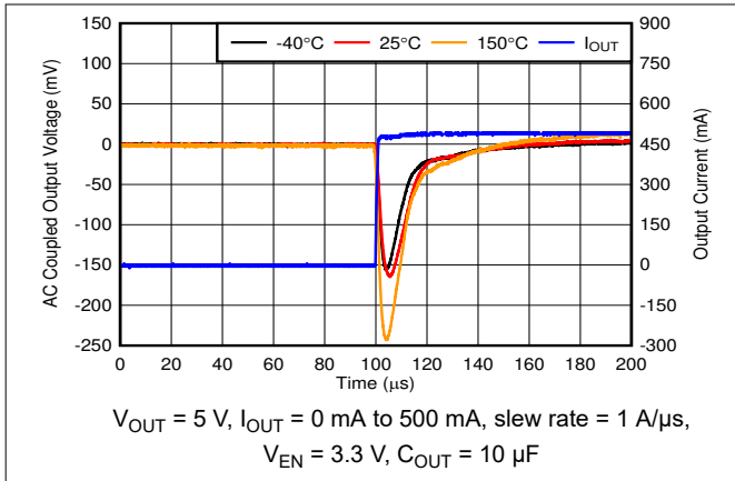
图 6-25. Load Transient, No Load to 500-mA Rising Edge
