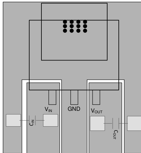
图 10-1. KVV Package Fixed Output
