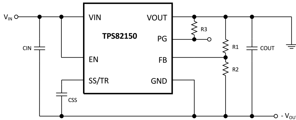
图 30. Inverting Power Supply Schematic
