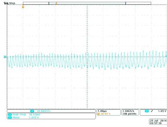
Figure 39. Output Voltage Ripple for TPS8268105 (Vin = 5V, Vout = 1.05V, Iout = 900mA)
