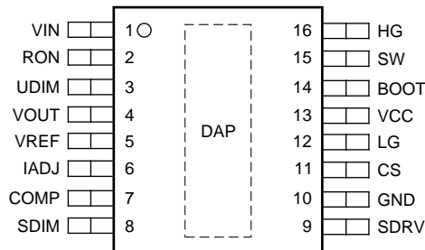
TPS92641 PWP Package 16-Pin HTSSOP Top View
