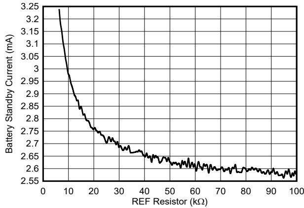
Figure 5-1. Standby Current vs REF Resistor
