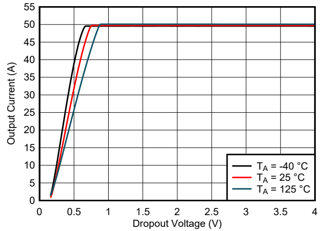
Figure 5-4. Output Current vs Dropout Voltage
