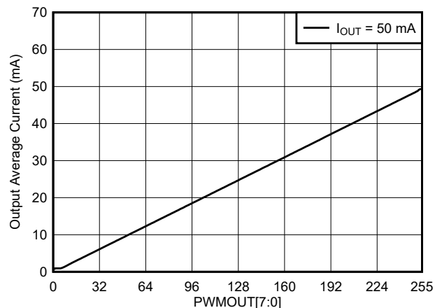
Figure 5-6. Average Current vs PWMOUT[7:0]
