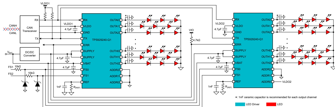
Figure 7-2. Typical Application Schematic
