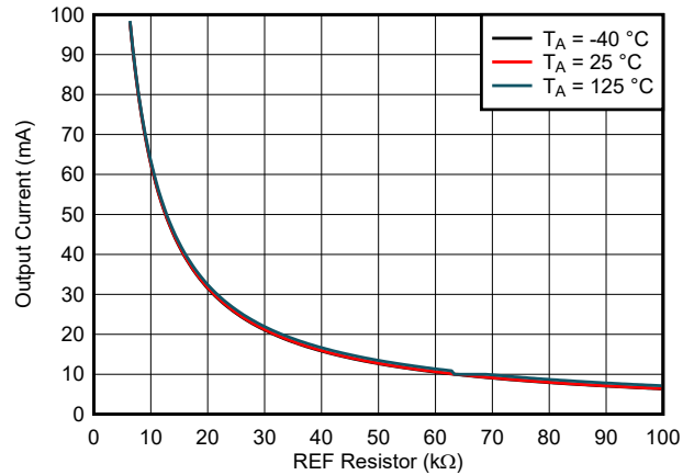
Figure 5-2. Output Current vs REF Resistor
