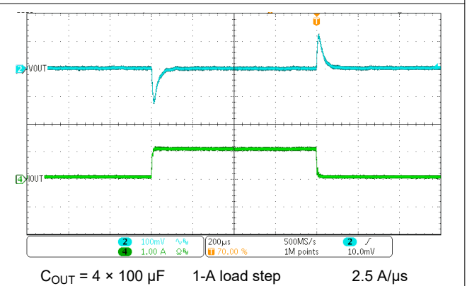
图 9-5. Transient Response Waveform
