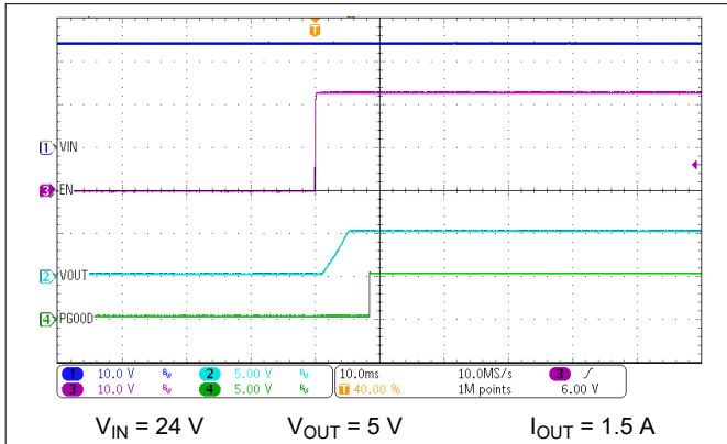
图 9-2. Start-up Waveforms
