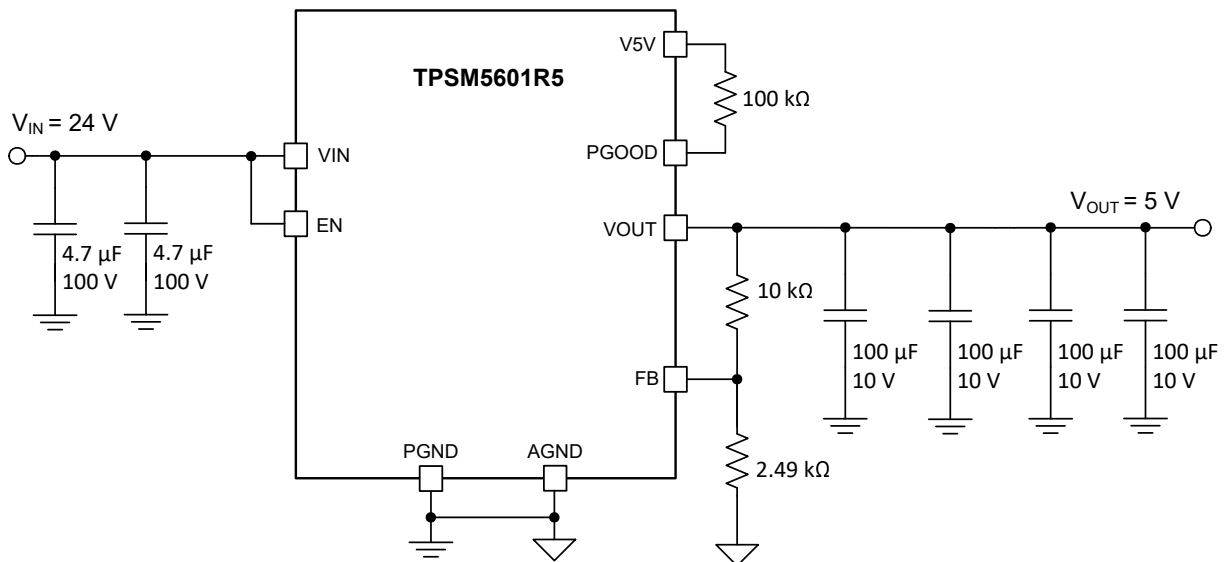
图 9-1. TPSM5601R5 Typical Schematic
