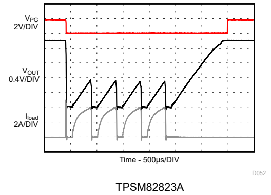
图 9-160. Short Circuit, HICUP Protection Entry / Exit
