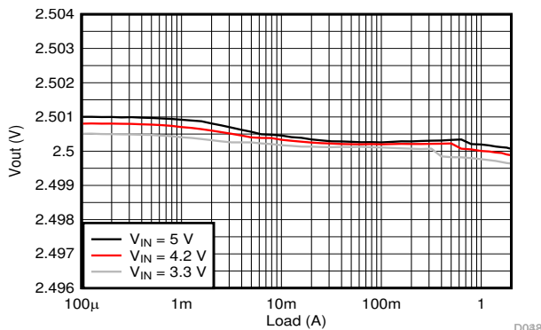
图 9-67. Load Regulation
