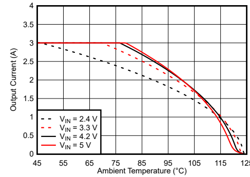
V_{OUT} = 1.8\text{ V} TPSM82823A R_{\theta JA} = 64.3^\circ\text{C/W}
