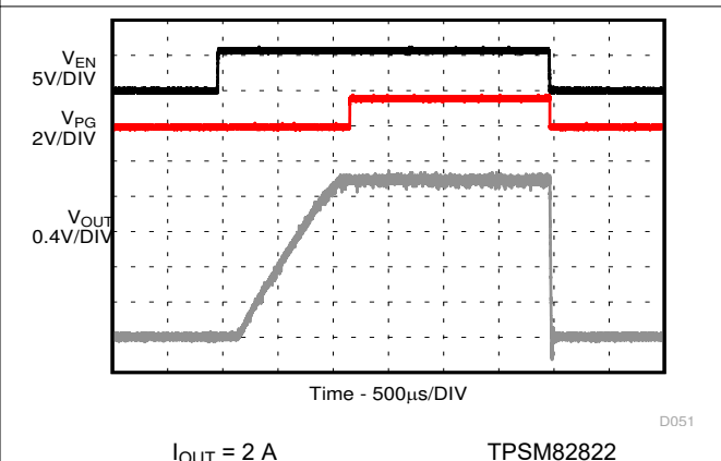
图 9-82. Start-up / Shutdown with Resistive Load
