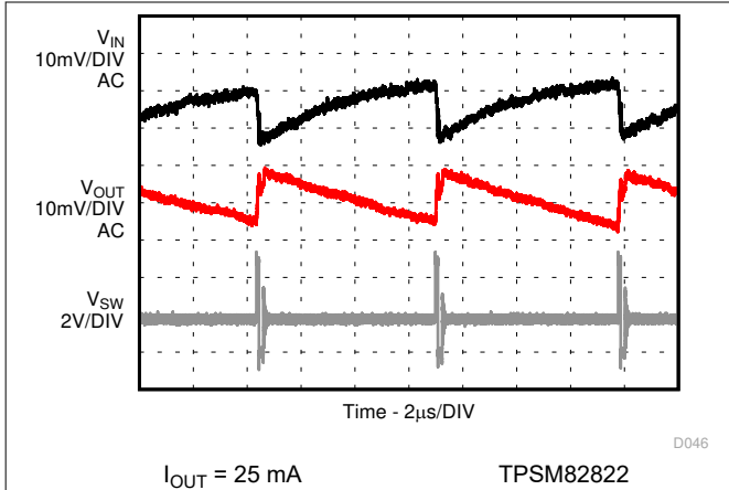
图 9-77. Input and Output Ripple in PSM Mode
