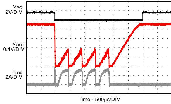
图 9-83. Short Circuit, HICCU Protection Entry / Exit
