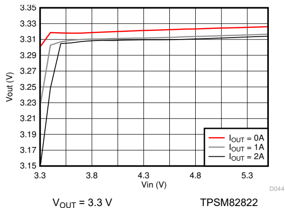
图 9-75. Line Regulation
