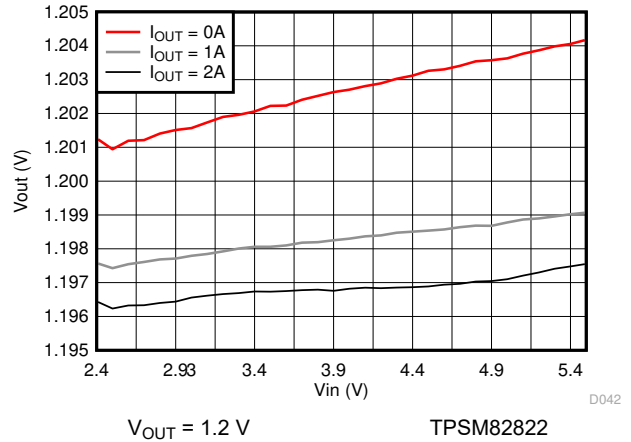
图 9-72. Line Regulation
