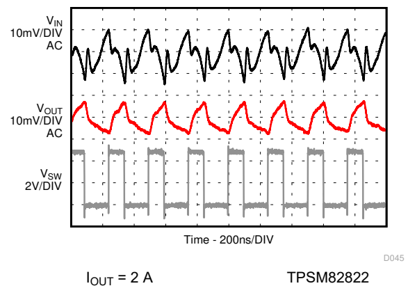
图 9-76. Input and Output Ripple in PWM Mode
