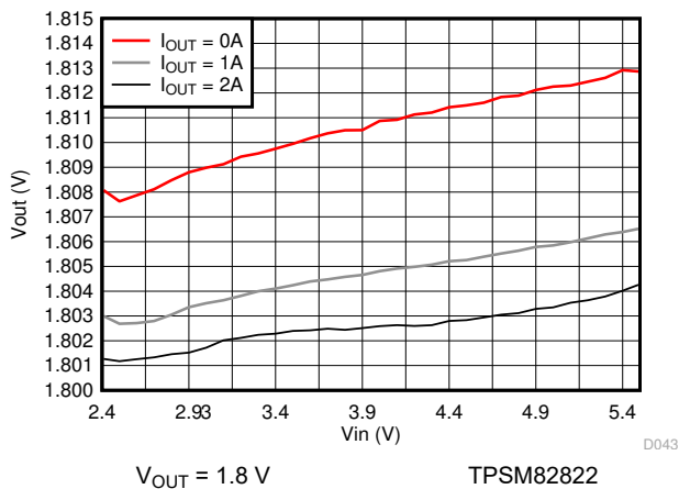
图 9-73. Line Regulation
