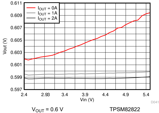
图 9-71. Line Regulation
