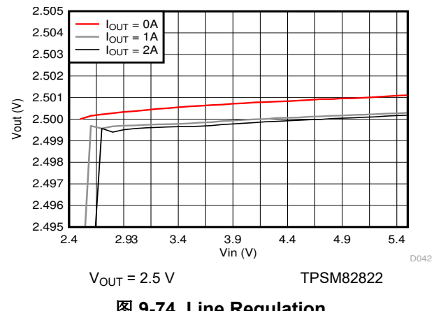
图 9-74. Line Regulation
