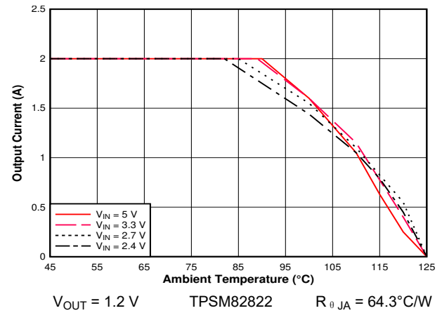
图 9-62. Safe Operating Area
