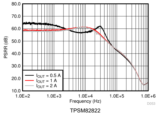
图 9-85. Power Supply Rejection Ratio (PSRR)
