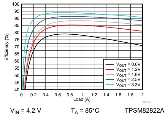
图 9-89. Efficiency
