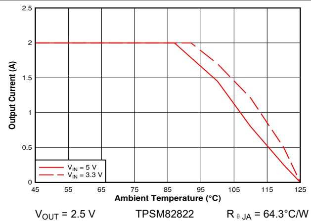
图 9-64. Safe Operating Area
