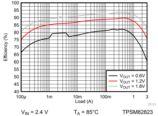
图 9-117. Efficiency
