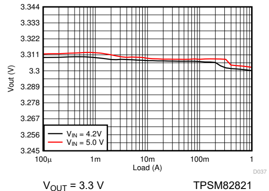
图 9-20. Load Regulation
