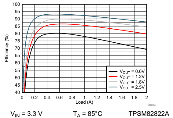
图 9-91. Efficiency
