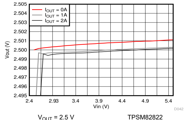
图 9-74. Line Regulation
