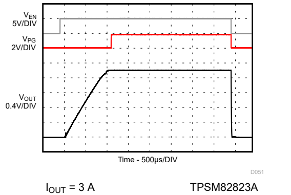
图 9-159. Start-up / Shutdown with Resistive Load
