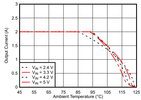
V_{OUT} = 1.8\text{ V} TPSM82822A
