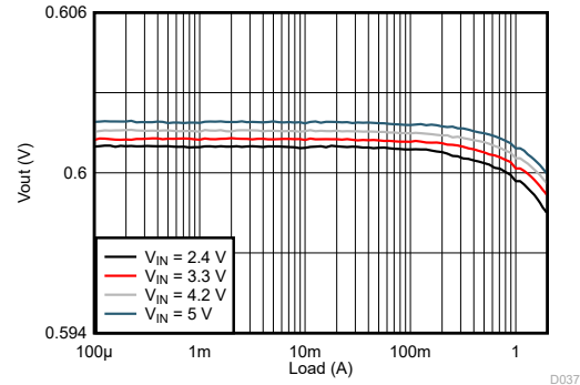
V_{OUT} = 0.6\text{ V} TPSM82822A
