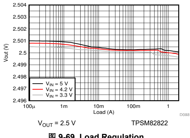
图 9-69. Load Regulation
