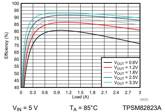
图 9-138. Efficiency
