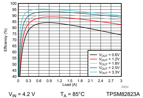
图 9-140. Efficiency
