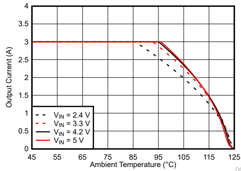
V_{OUT} = 0.6\text{ V} TPSM82823A R_{\theta JA} = 64.3^\circ\text{C/W}
