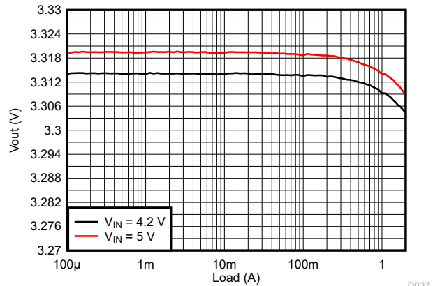
V_{OUT} = 3.3\text{ V} TPSM82822A
