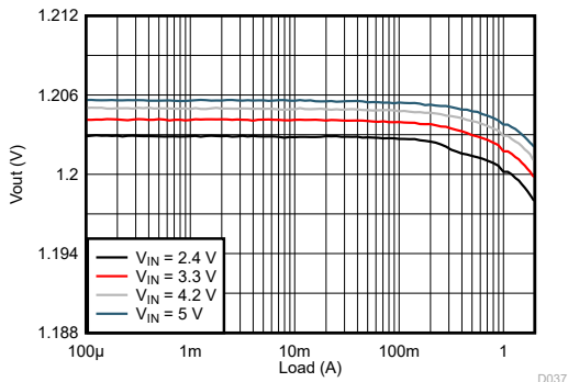
V_{OUT} = 1.2\text{ V} TPSM82822A
