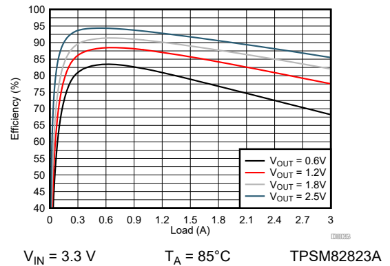
图 9-142. Efficiency
