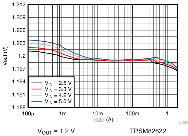
图 9-67. Load Regulation
