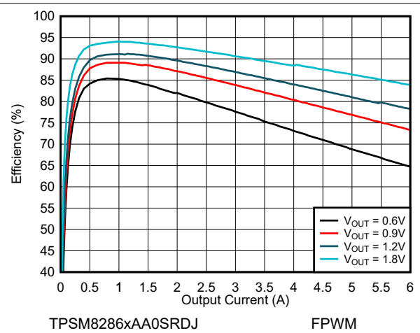
图 9-7. Efficiency V_{IN} = 2.8\text{ V} and T_A = 85^\circ\text{C}
