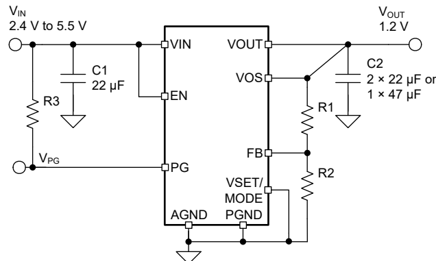
Figure 9-1. Typical Application
