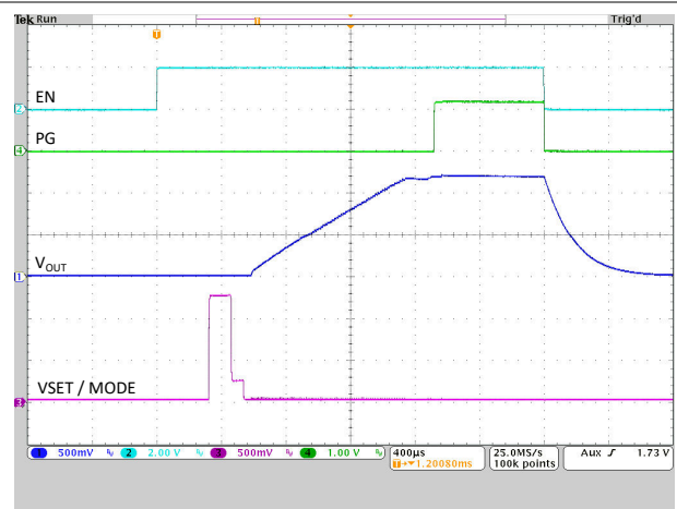
R_{VSET} = 56.2 \text{ k}\Omega I_{OUT} = 0 \text{ A} Figure 9-27. Start-Up with No Load
