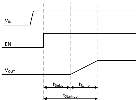
Figure 8-2. Start-Up Sequence
