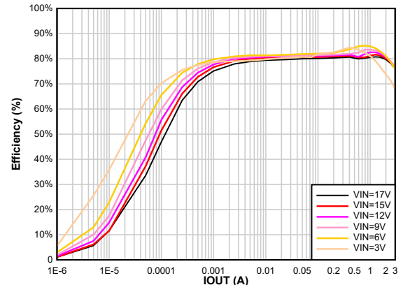
Figure 8-6. Efficiency vs Output Current V_{OUT} = 1.2 \text{ V}
