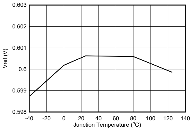
Figure 7-7. VREF Voltage
