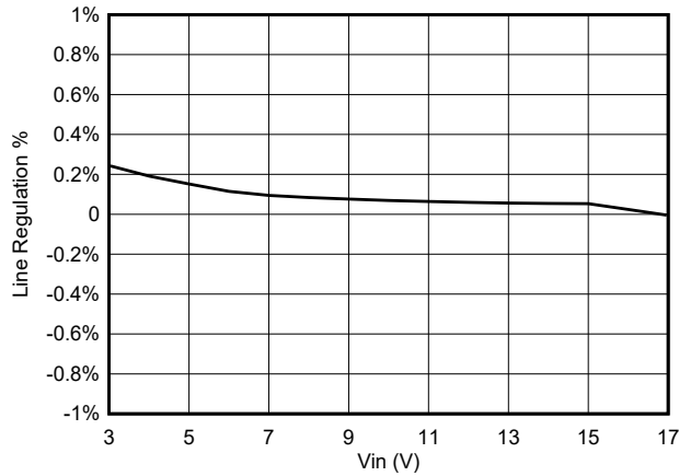
Figure 9-4. TPSM863252 Line Regulation vs V_{IN} at 3-A Loading
