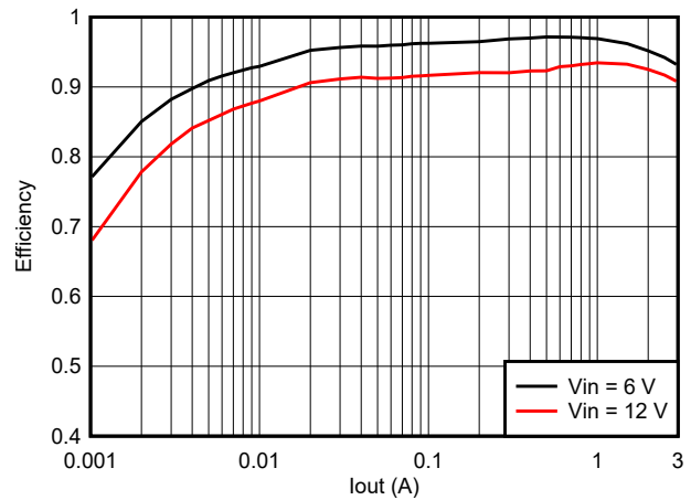
Figure 7-14. TPSM863252 Efficiency at 5 V OUT
