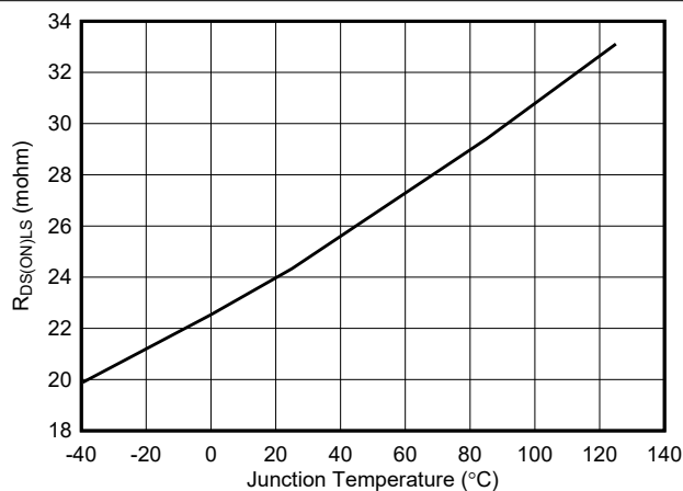
Figure 7-5. Low-Side R_{DS(ON)}
