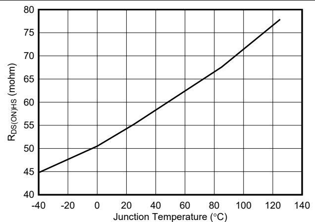
Figure 7-6. High-Side R_{DS(ON)}
