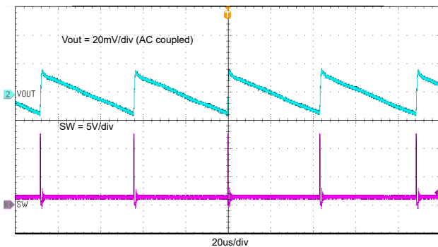
Figure 9-6. TPSM863252 Output Voltage Ripple With 0.01-A Loading
