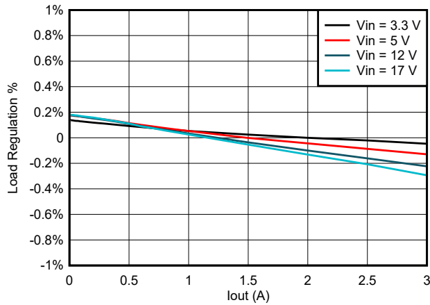
Figure 9-2. TPSM863252 Load Regulation vs Loading
