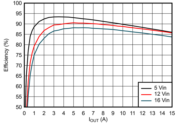
图 8-5. Efficiency
