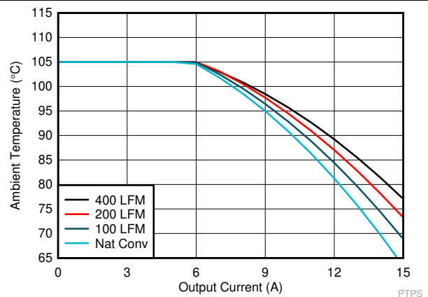
图 6-6. SOA, 5Vin 1.0V out_IN , 600 KHz, FCCM, Internal VCC LDO
