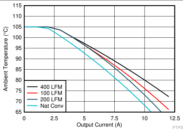
图 6-5. SOA, 12 V 5.0V out_IN , 600 KHz, FCCM, Internal VCC LDO
