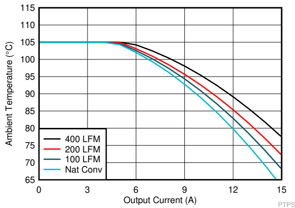
图 6-3. SOA, 12 V 1V out_IN , 600 KHz, FCCM, Internal VCC LDO
