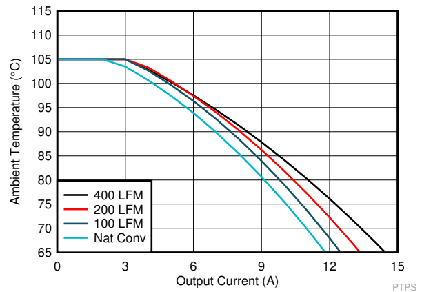
图 6-4. SOA, 12 V 3.3V out_IN , 600 KHz, FCCM, Internal VCC LDO
