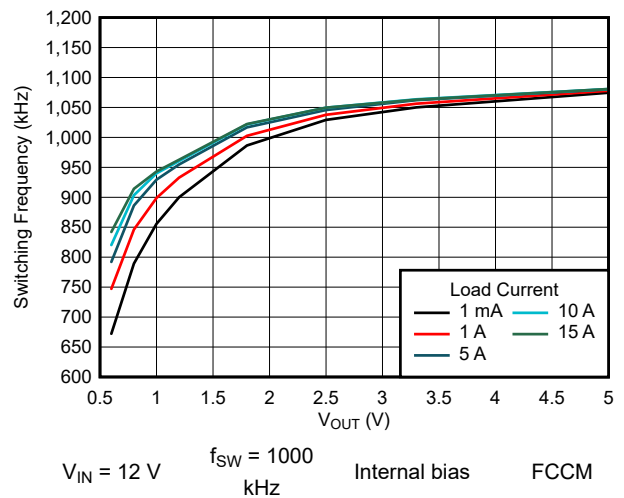
图 8-25. Switching Frequency
