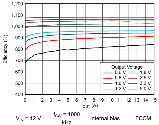
图 8-23. Switching Frequency
