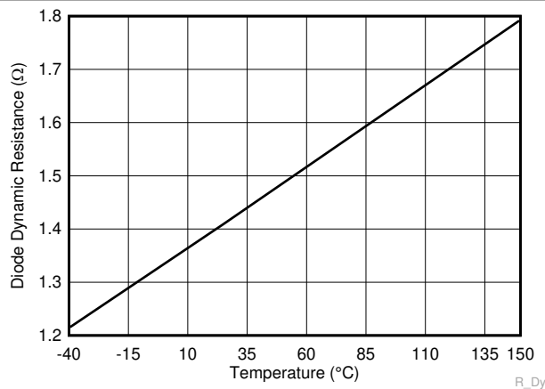
图 6-17. Boot Diode Dynamic Resistance
