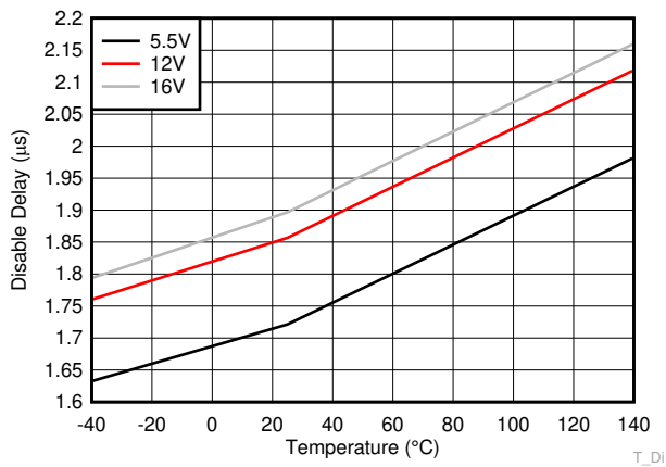
图 6-13. Disable Delay
