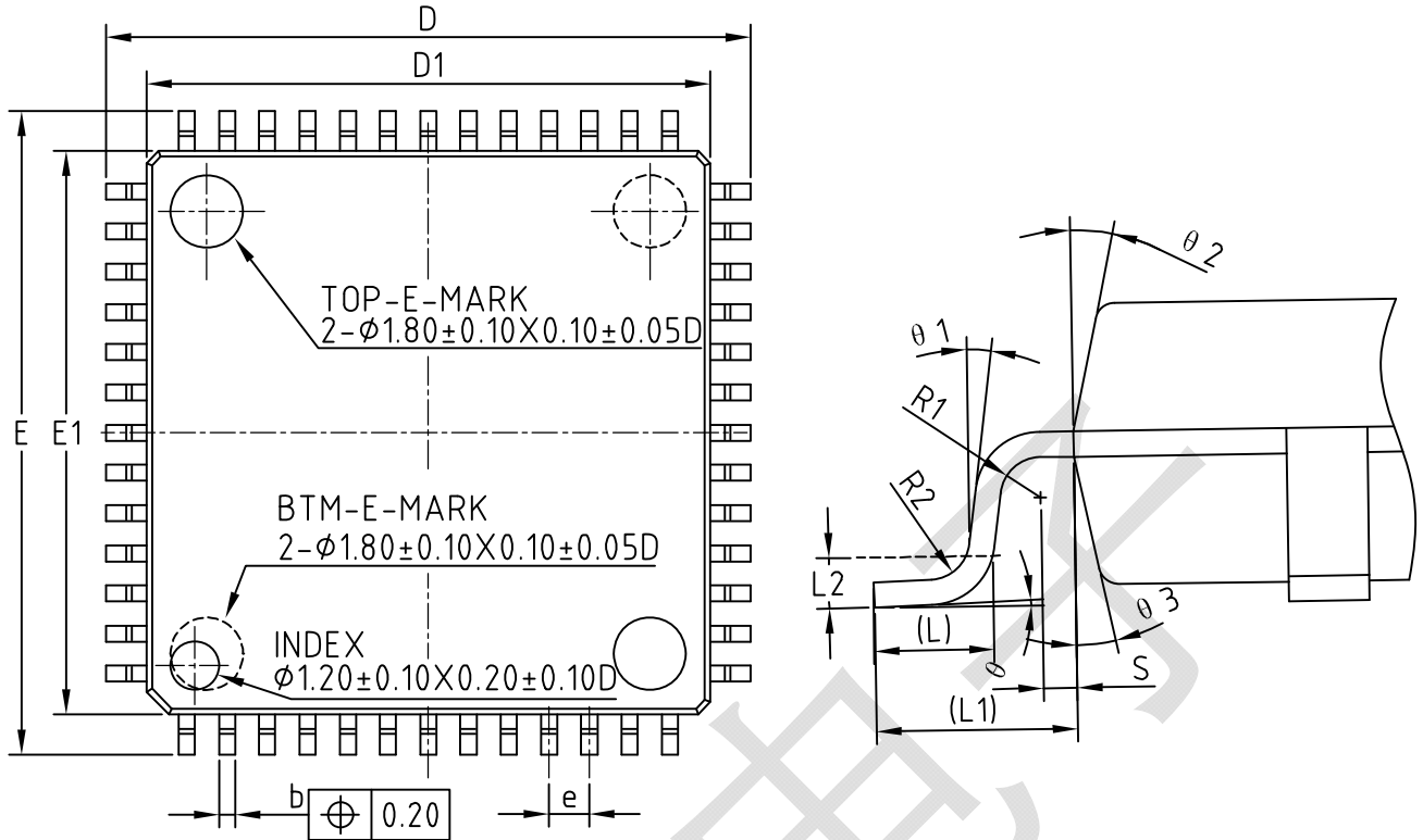
封装示意图 (LQFP52 14mm*14mm)
