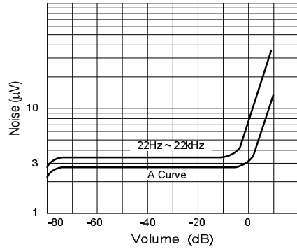
Fig.4 Noise vs. Volume/Gain settings
