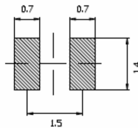
LAND PATTERN<REFERENCE>
