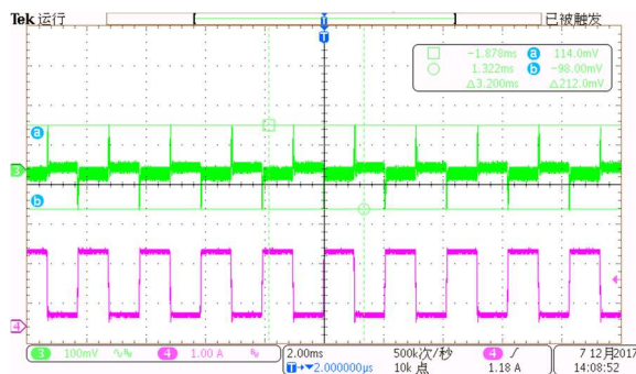
Load transient(0.2A-1.8A-0.2A)
