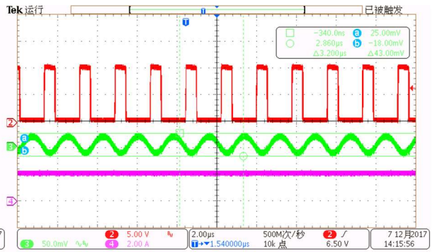
Iout=100% load
