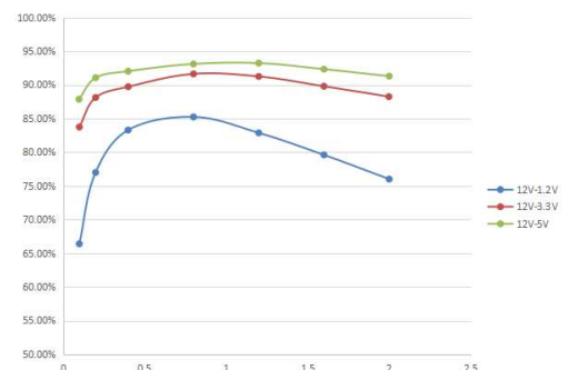
2. Efficiency(%) vs. Load Current(A)
