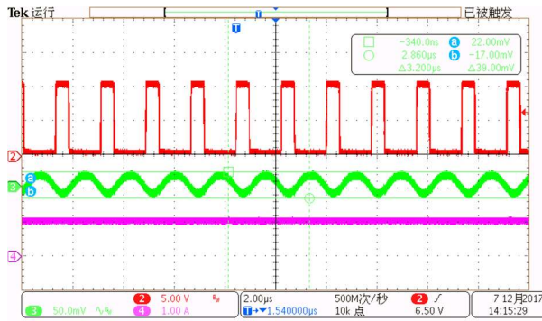
Iout=50% load
