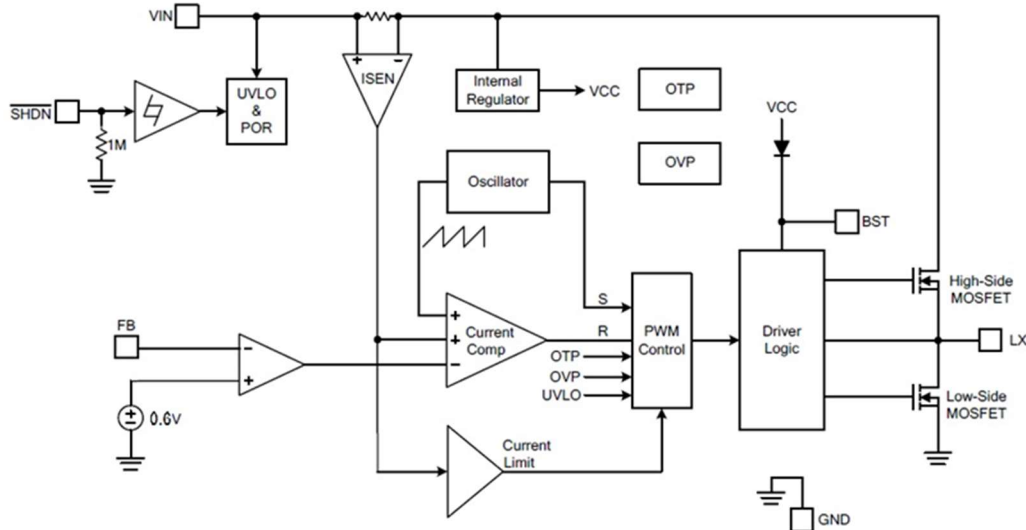
Figure 3. STI3470L Block Diagram
