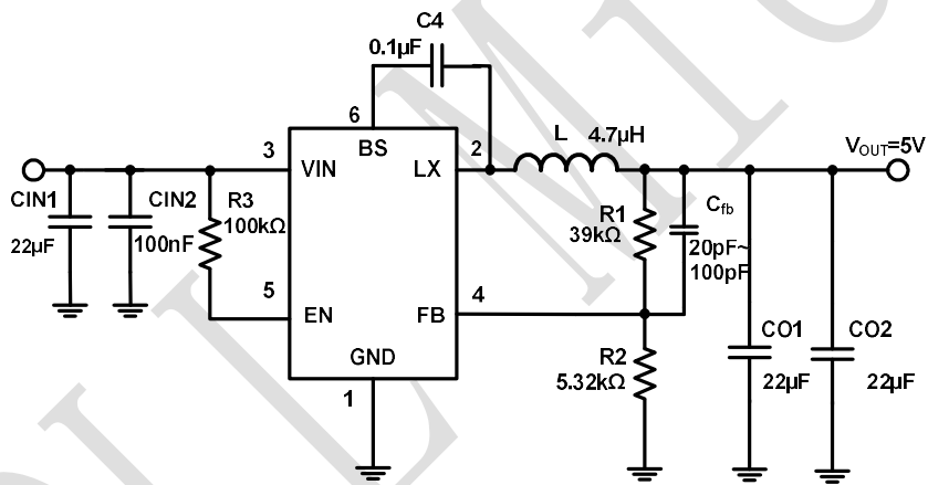
Figure 4. 12V IN , 5V Output ( V_{FB}=0.6V )
