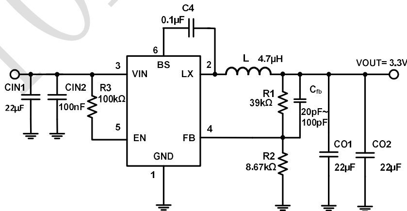
Figure 5. 12V IN , 3.3V Output ( V_{FB}=0.6V )
