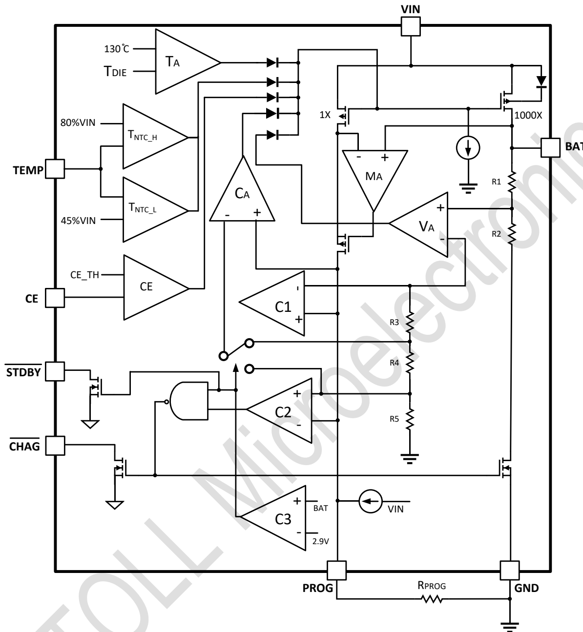
Figure 2. TMI4056E and TMI4056EH Block Diagram
