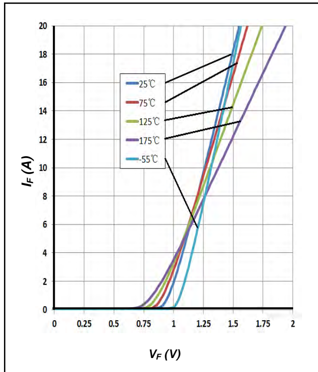
Figure 1. Forward Characteristics
