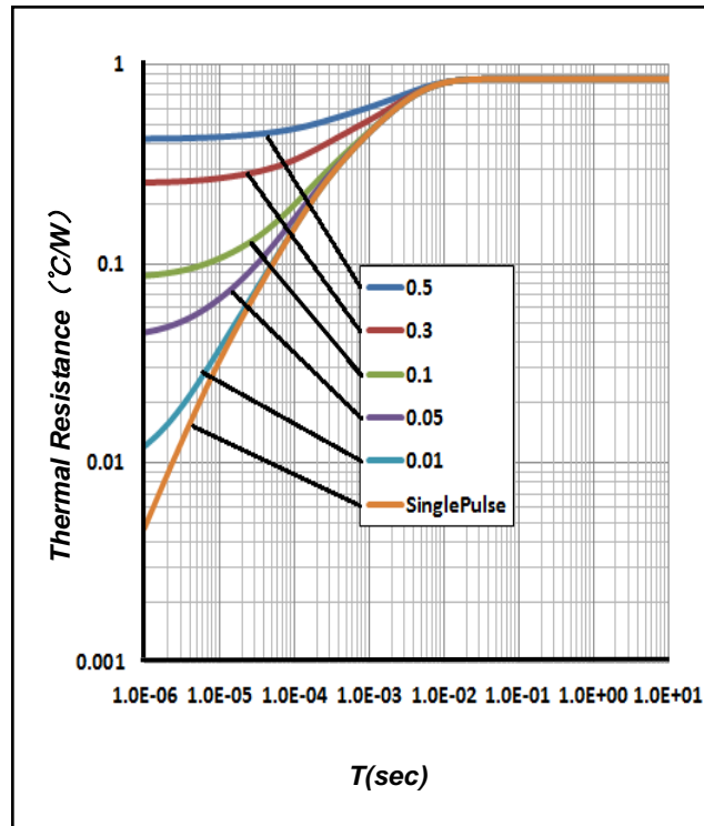
Figure 9. Transient Thermal Impedance
