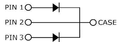
TO-247-3 (1)(2)(3)
