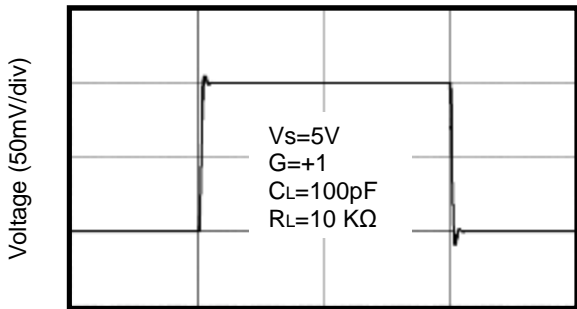
Time (1μs/div)
