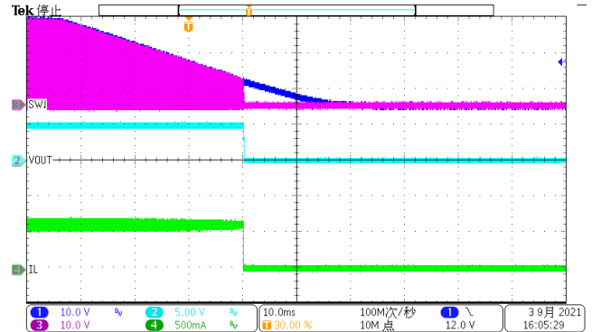
Figure 12. Power down(Iload=0.6A)
