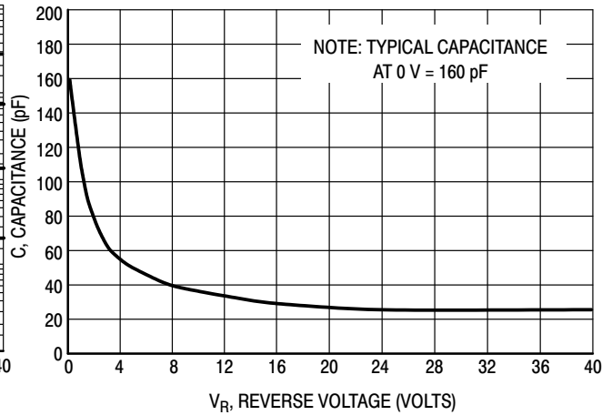
Figure 4. Typical Capacitance
