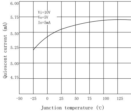
Fig.14 Quiescent current
