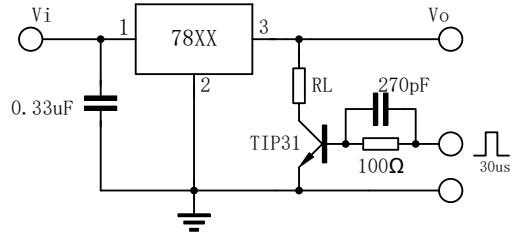
FIG.2 LOAD REGULATION
